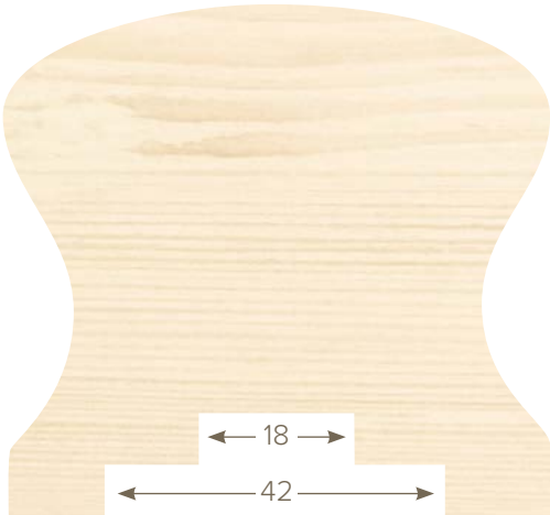
Ladies Waist H3.2 Primed Pine 63 x 65
